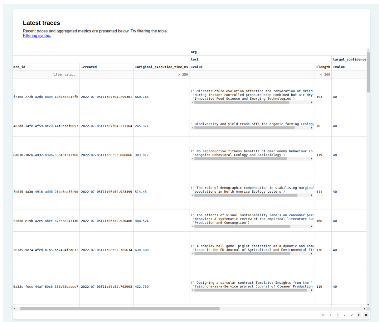
Figure 5.11: A dynamically updating, tabular view of traces matching a user-defined filter. Useful for exploring historical predictions or debugging the cause of exceptions (which are also searchable). The filters set in the table affect the other diagrams of the dashboard.
